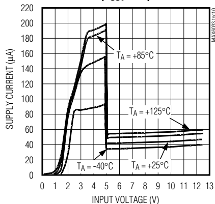
SUPPLY CURRENT vs. INPUT VOLTAGE ( V_{OUT} = 5V )
