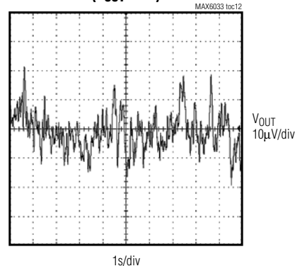
0.1Hz TO 10Hz OUTPUT NOISE ( V_{OUT} = 5V )
